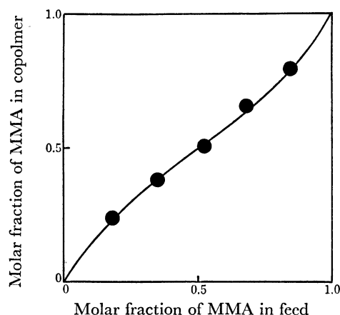
Fig. 6. Monomer-copolymer composition curve. (MMA+St) 6 cm 3 , ETTT 0.1 cm 3 , H 2 O 3 cm 3 , FeCl 3 ·6H 2 O 0.06 g; 85 °C, 6 h.
